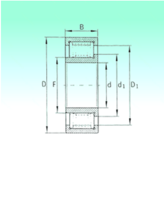
ZSL192305 Bearing 2D drawings and 3D CAD models
